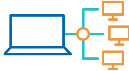
Workflow Applications
